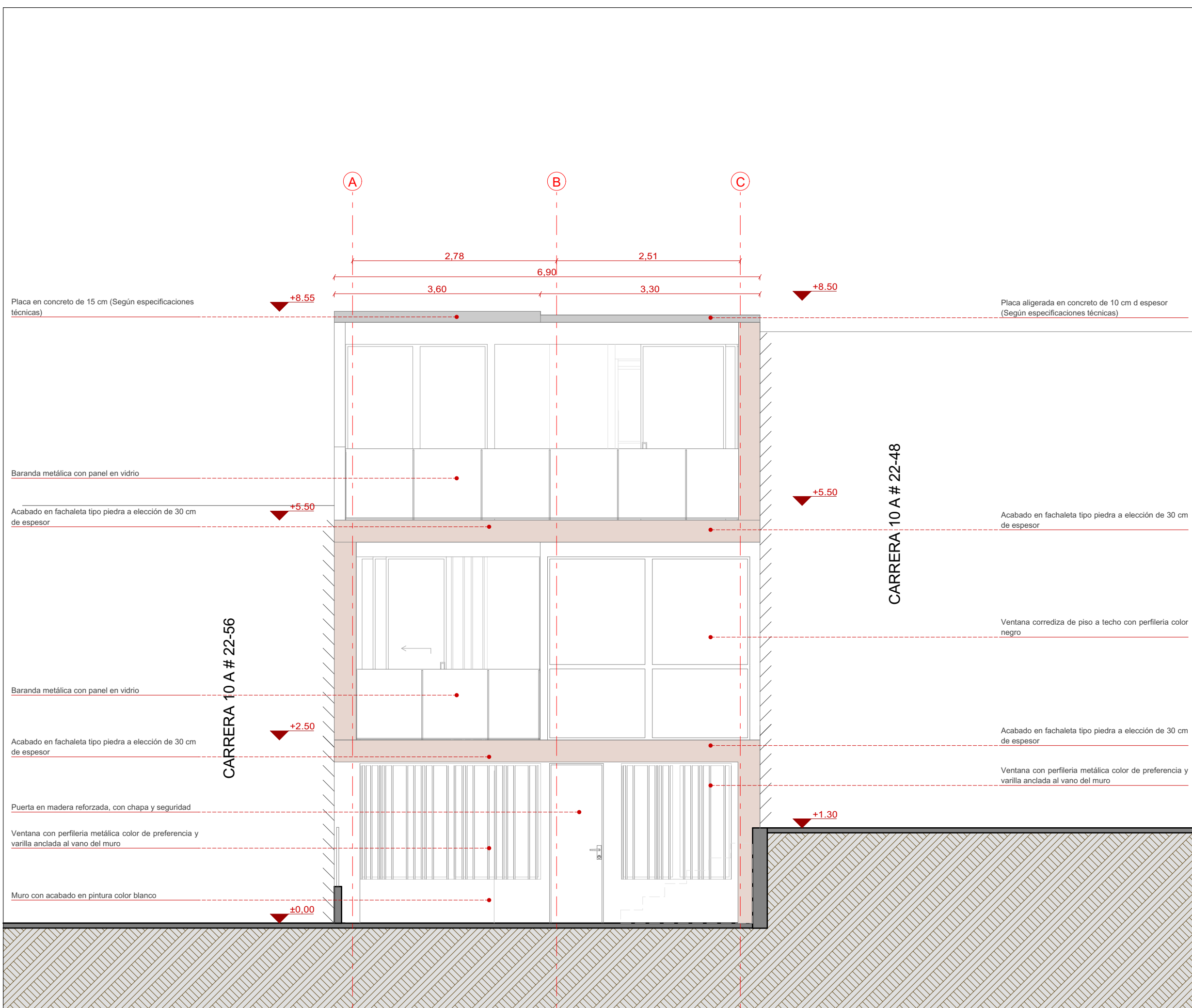
Fachada Principal
